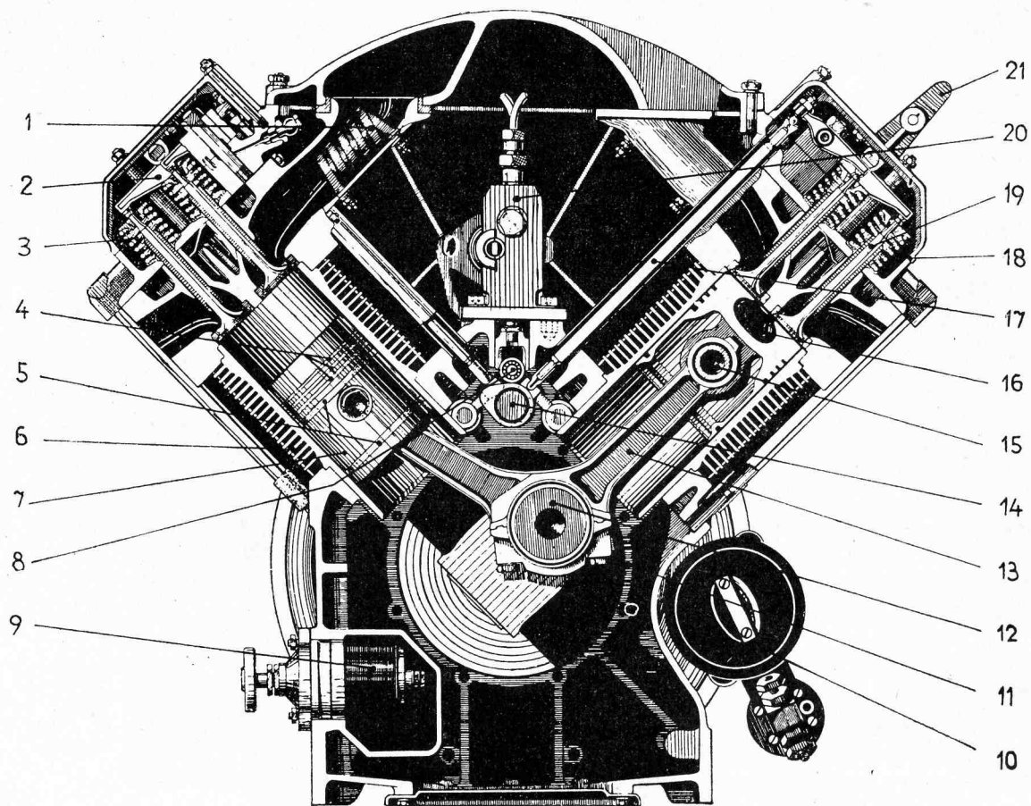
Obr. 2-5 Motor FD 21/1
